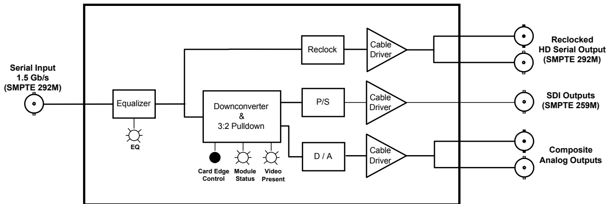
Figure 1: 2410MD Block Diagram
