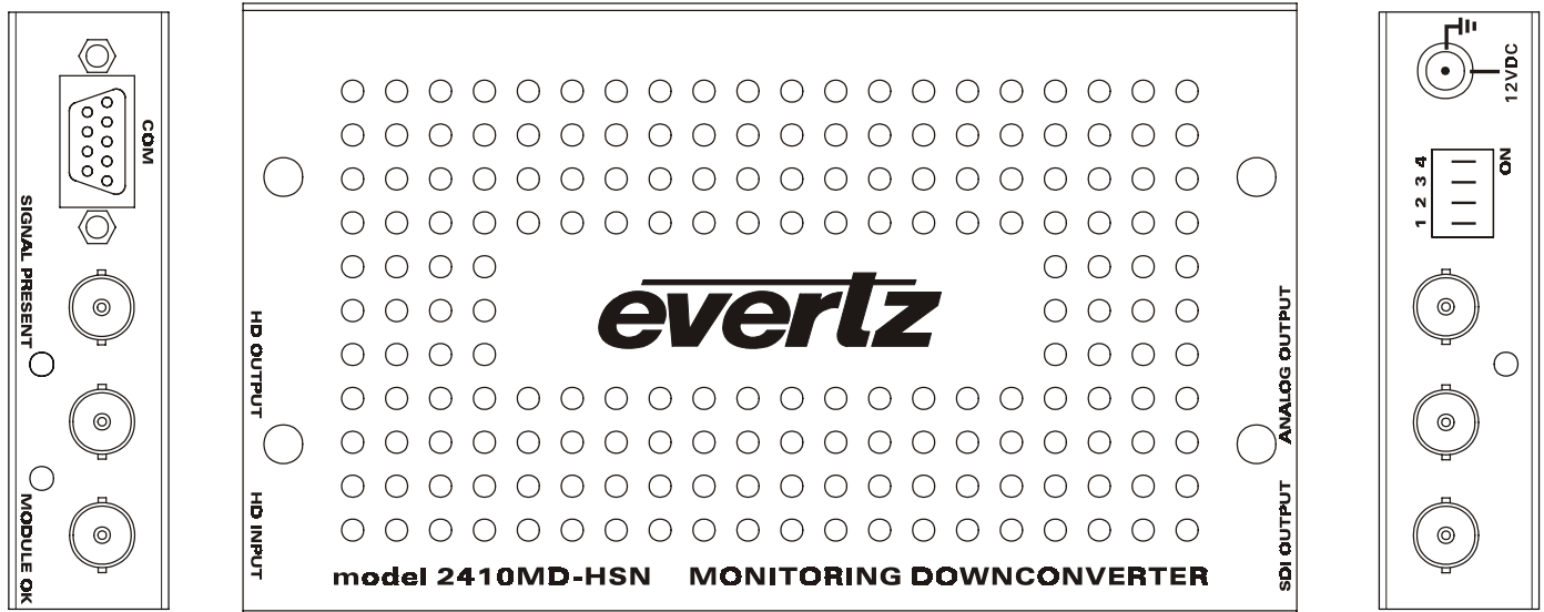
Figure 2: 2410MD-HSN Module
